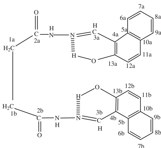
Figure 1. Structure along with numbering scheme of H_4nsh .
